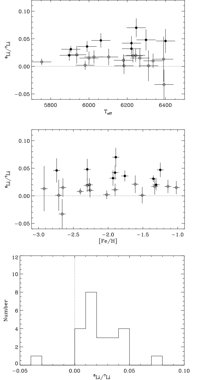
FIG. 13.— Derived {}^6\text{Li}/{}^7\text{Li} as a function of T_{\text{eff}} (Upper panel) and [\text{Fe}/\text{H}] (Middle panel). The stars considered to have a significant detection ( \geq 2\sigma ) of {}^6\text{Li} are shown as solid circles while non-detections are plotted as open circles. Note that the non-detections do not cluster around {}^6\text{Li}/{}^7\text{Li} = 0.00 but rather at \approx 0.01 . This is also illustrated as a histogram (Lower panel). The observed distribution is clearly not representative of a Gaussian centered at {}^6\text{Li}/{}^7\text{Li} = 0.00 .
